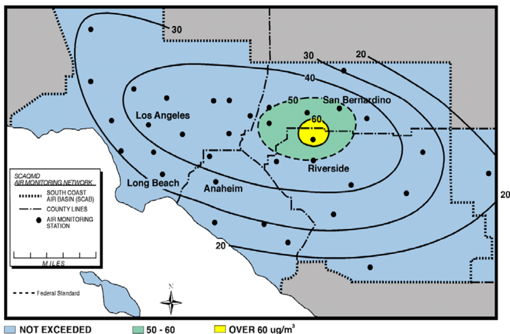
FIGURE 2-12 Suspended Particulate Matter (PM 10 ) - 2001 Annual Arithmetic Mean, \mu\text{g}/\text{m}^3
