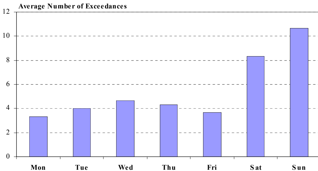
FIGURE 2-6 OZONE Day-of-Week Variation, 1999-2001 Exceedances of the Federal Standard by Day of Week
