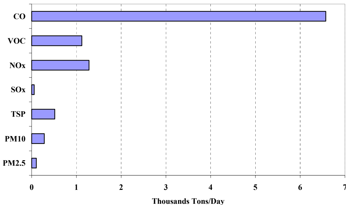
FIGURE 1-3 1997 Average Daily Emissions in the Basin
