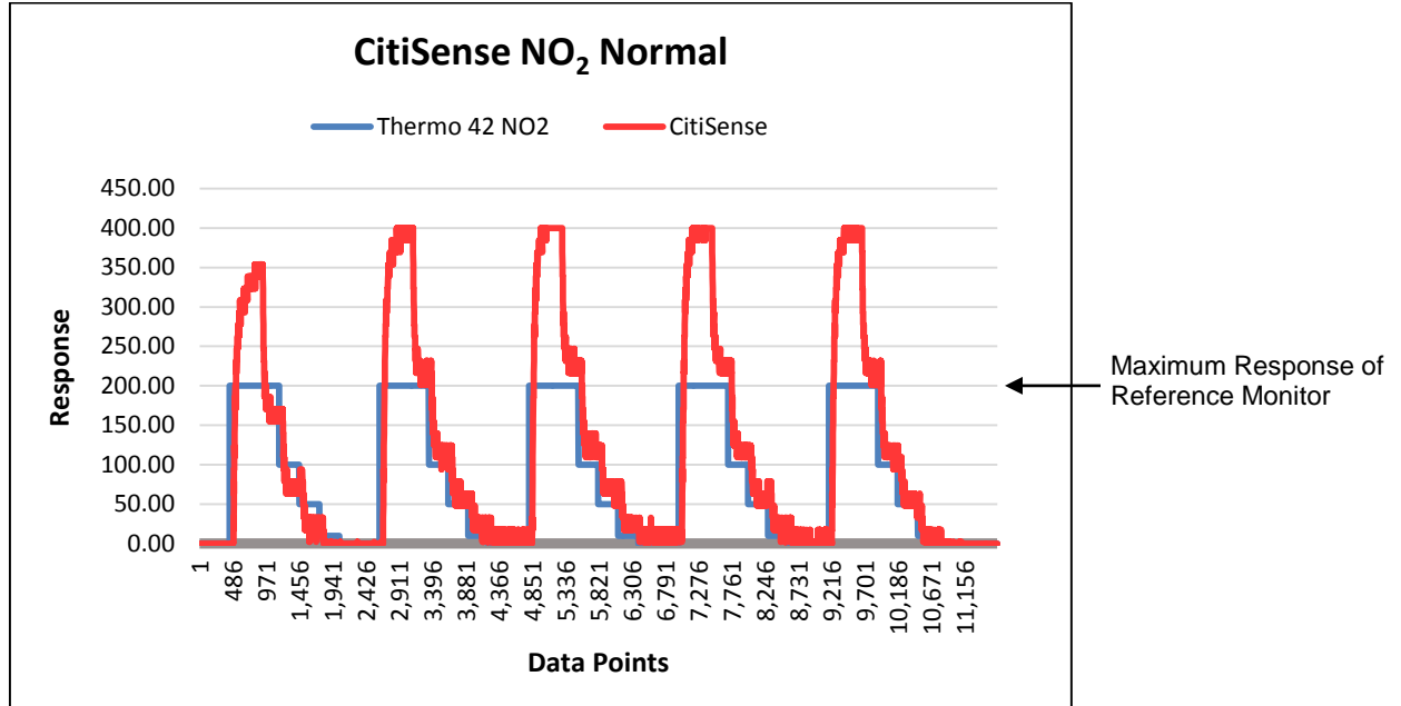
Figure 9. Example CitiSense Response for NO 2 under Normal Challenge Conditions
