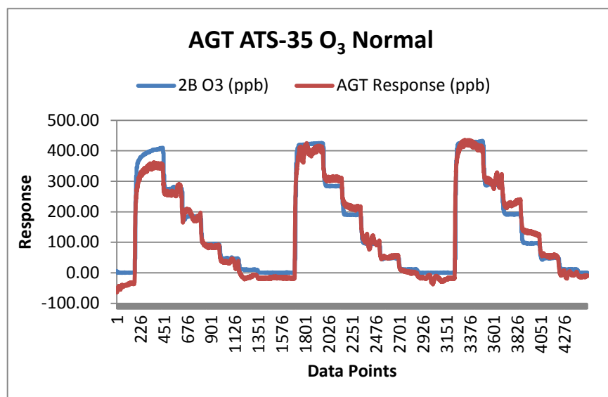
Figure 2. Example AGT ATS-35 Response for O 3 under Normal Challenge Conditions
