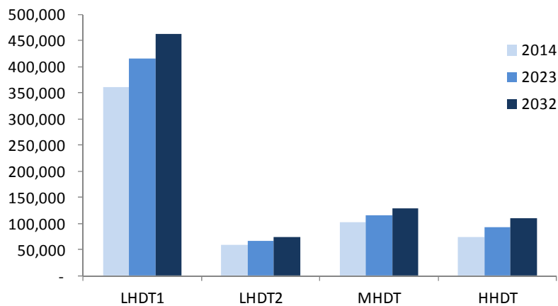
Figure 7. Populations for Specific On-Road Heavy-Duty Vehicles*
