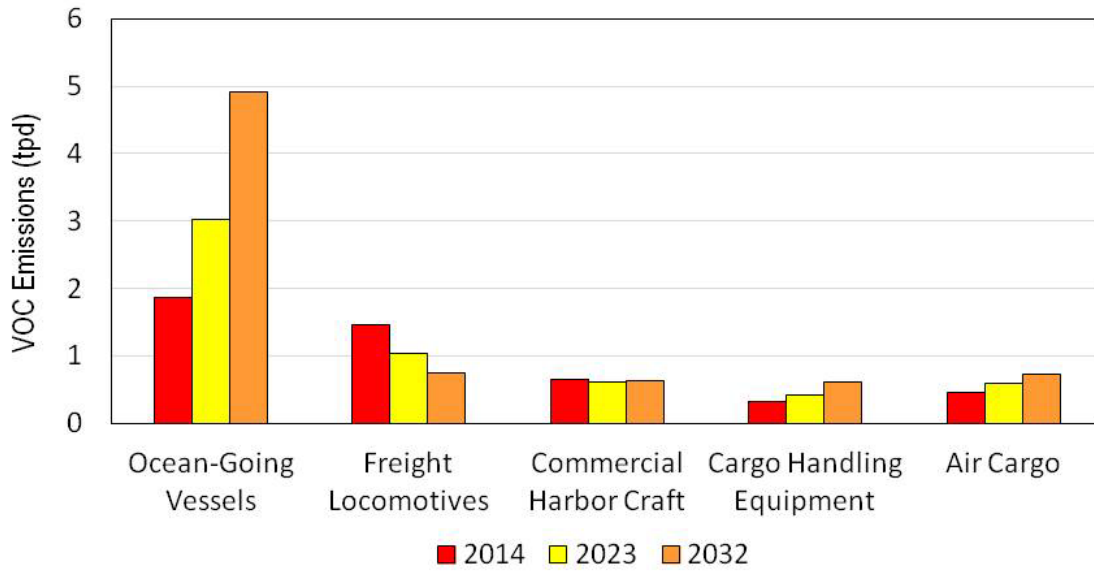
Figure 9. VOC Emissions for Specific Off-Road Goods Movement Sources*
