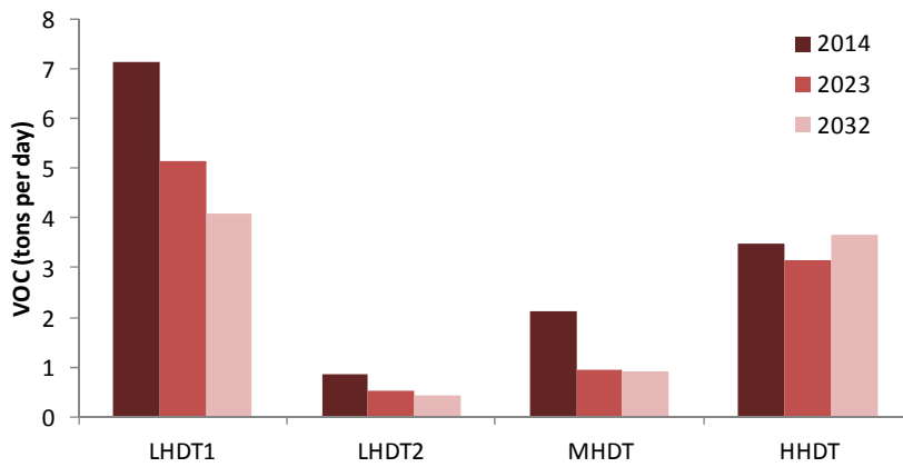
Figure 6. VOC Emissions for Specific On-Road Heavy-Duty Vehicles*
