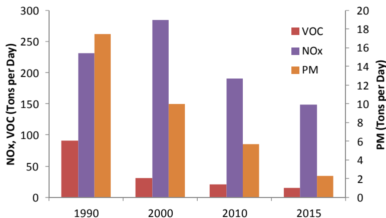
Figure 4. On-Road Heavy-Duty Truck Emissions in the South Coast Air Basin *
