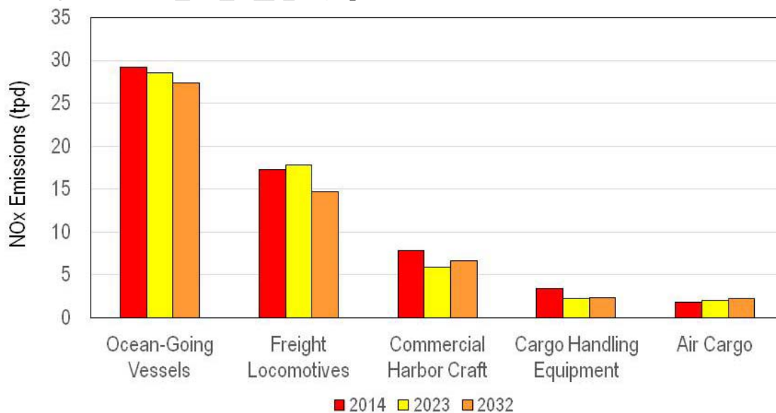
Figure 8. NOx Emissions for Specific Off-Road Goods Movement Sources*
