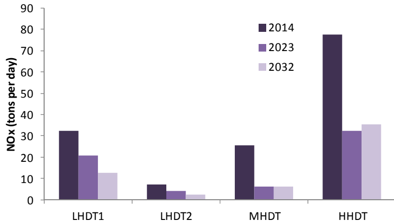
Figure 5. NOx Emissions for Specific On-Road Heavy-Duty Vehicles*
